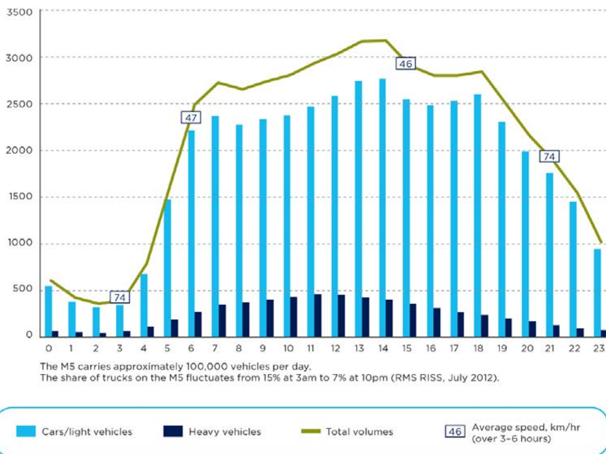
Figure 8 M5 hourly traffic volumes, average day 2011. West bound lanes of traffic at Kingsgrove weigh-in-motion (WIM) counter
