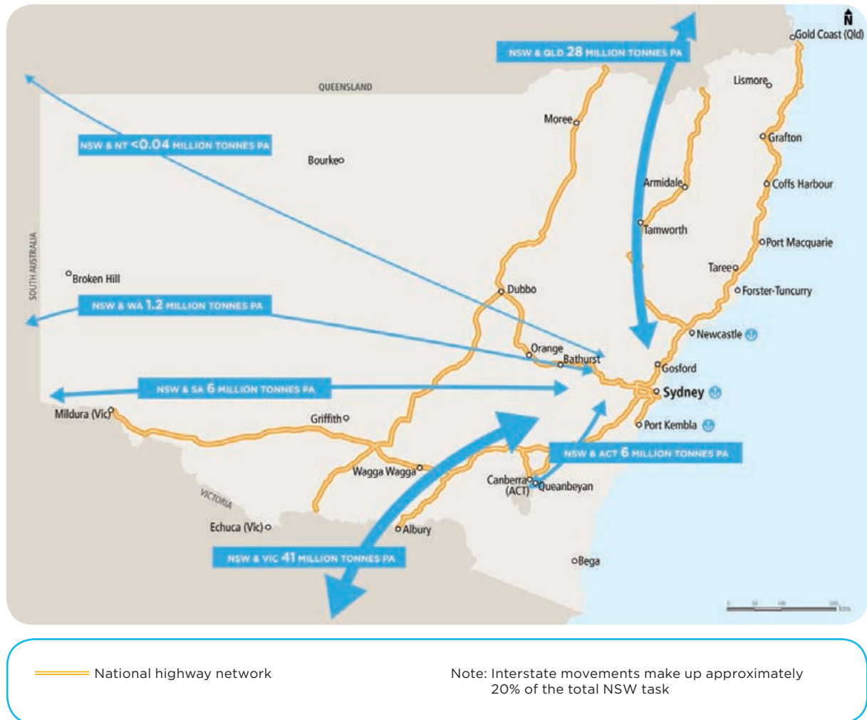
Figure 43 Interstate freight movements in 2011
