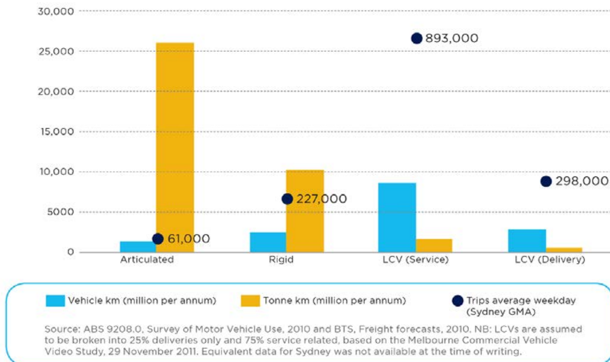
Figure 19 Comparison of truck and light commercial vehicle activity in NSW with trips on an average weekday
